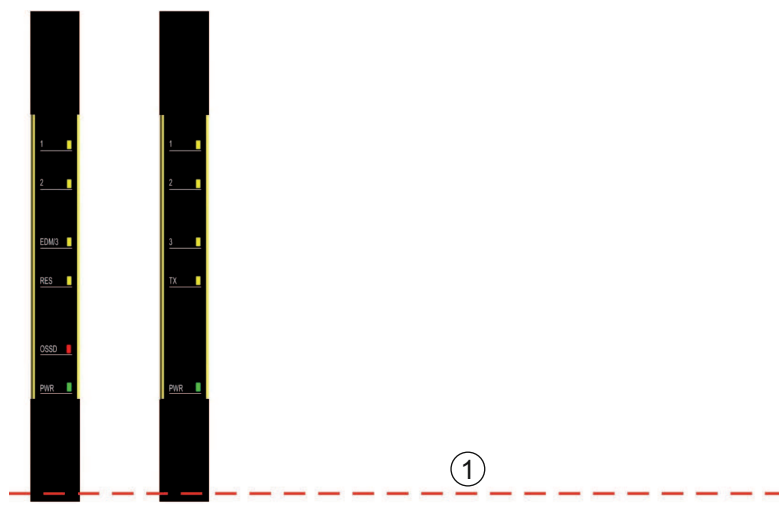
Fig. 8.1: Synchronization optics
