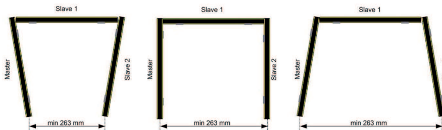
Fig. 8.3: Minimum distance for cascade system
