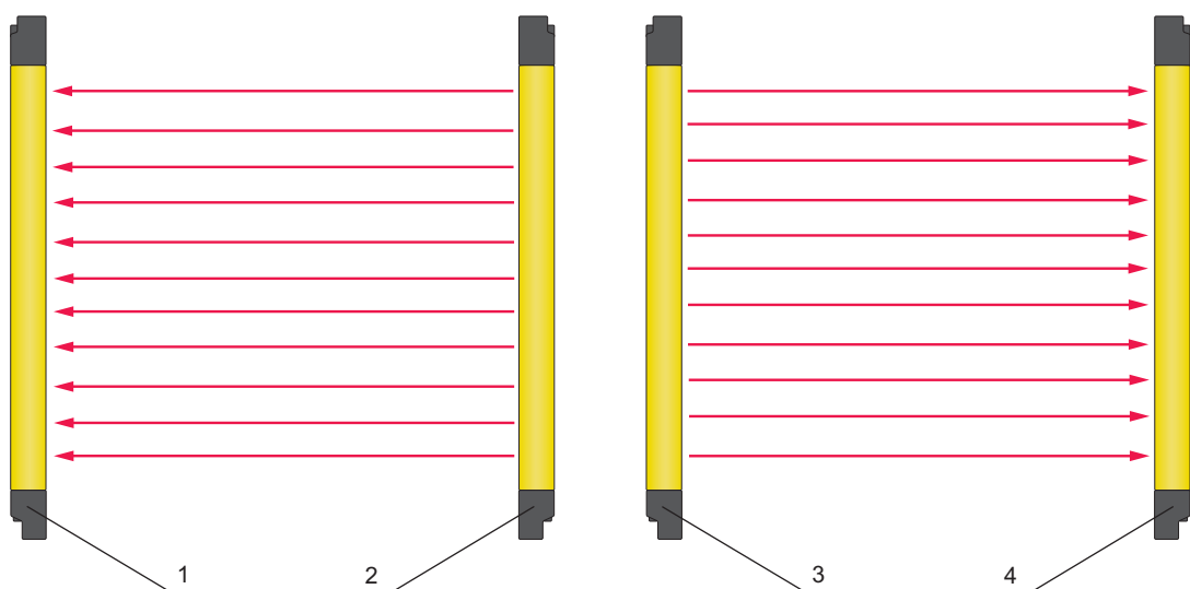
Fig. 6.5: Opposite mounting
