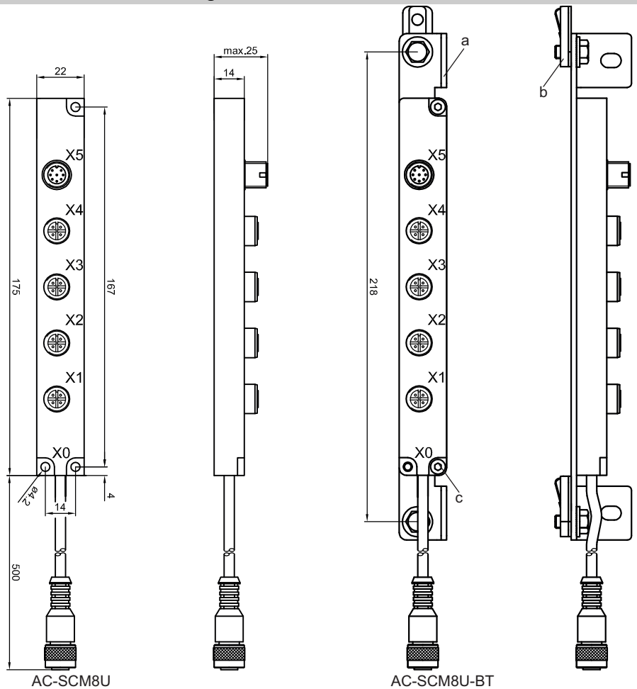
a = Mounting plate b = Sliding block c = M4x16 cheese head screw
