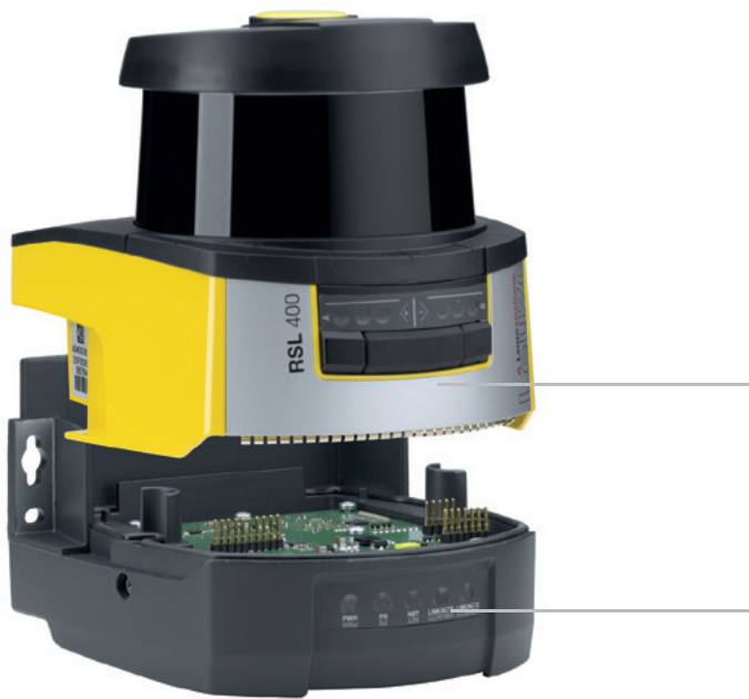
Scanner head with PROFIsafe function
